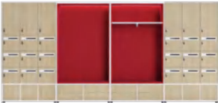
GG-ZHG-18 4836W*420D*2250H
