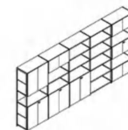
G-RFC-04 4122W*420D*1965H
