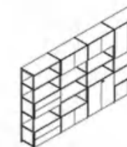
G-RFC-03 3300W*420D*1965H
