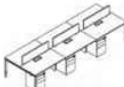
B-XST-S-03 3600W*1200D*750H 4200W*1200D*750H 4200W*1400D*750H 4500W*1400D*750H
