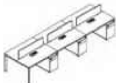
A-RIST-S-03 3600W*1200D*750H 4200W*1200D*750H 4200W*1400D*750H
