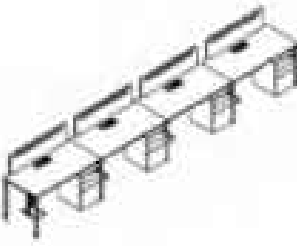
B-RST-D-04 4800W*600D*750H 5600W*600D*750H 5600W*700D*750H
