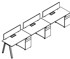
A-DST-D-03 3600W*600D*750H 4200W*600D*750H 4200W*700D*750H
