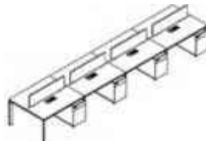
A-RIST-S-04 4800W*1200D*750H 5600W*1200D*750H 5600W*1400D*750H
