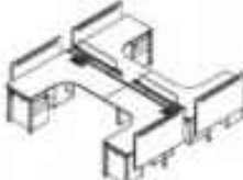
C-RST-工-03 2800W*2800D*750H 3000W*3000D*750H 3200W*3200D*750H
