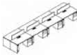
B-ANST-S-04 4800W*1200D*750H 5600W*1200D*750H 5600W*1400D*750H
